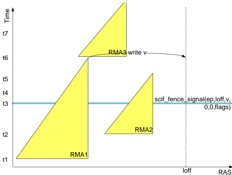
Figure 15: Using scif_fence_signal()
