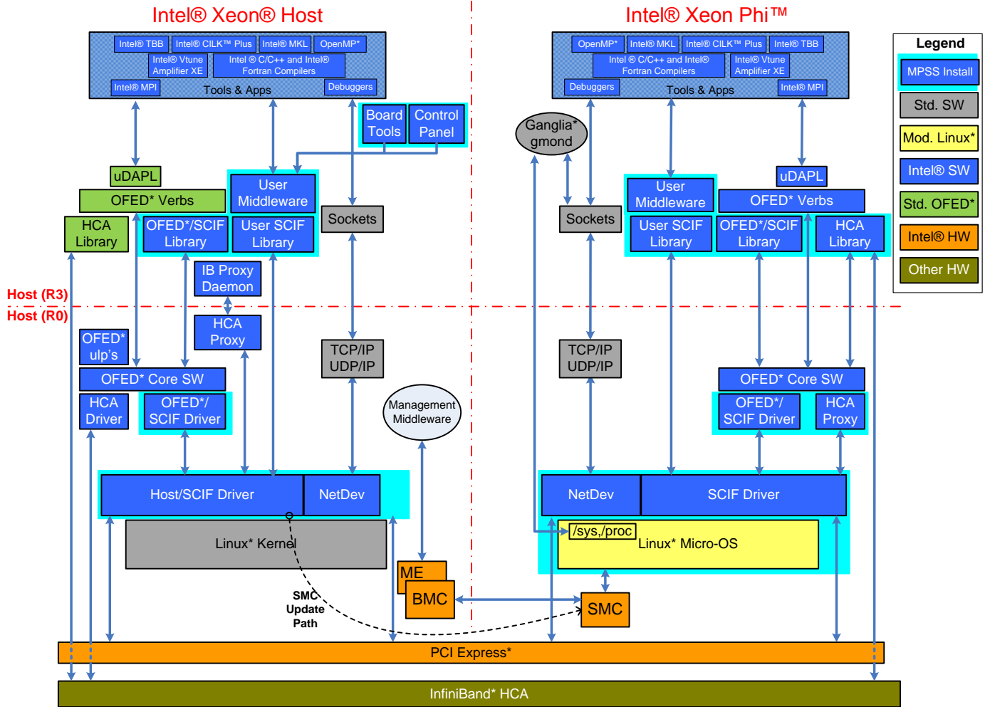
Figure 1: Intel® ManyCore Platform Software Stack (MPSS)
