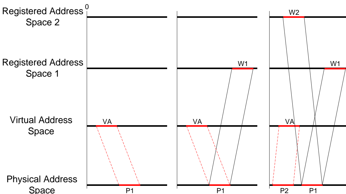
Figure 8: Registering windows using scif_pin_pages()
